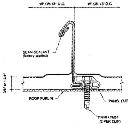
QUAD-LOK
