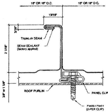
TRIP-LOK
